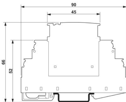
Dimensioned drawing
